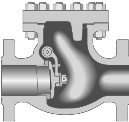
Figure 60-SF-U Flanged
