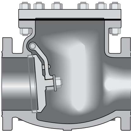
Figure 15-SF-U Flanged
