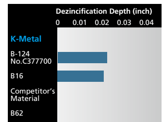
Fig. 4 Compared dezincification (to AS C316)
