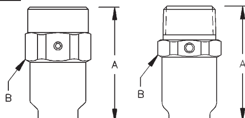
60° / 90° / 120° Female
