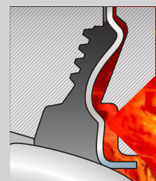
Seat retainer upstream
